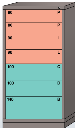
7 drawers, 77 compartments No. 250-680G-3 Single Drawer Access No. 251-680G-3 Multiple Drawer Access
