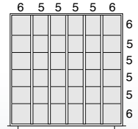
(H) 36 compartments 3 1/2"w x 3 1/2"d to 4 1/4"w x 4 1/4"d
