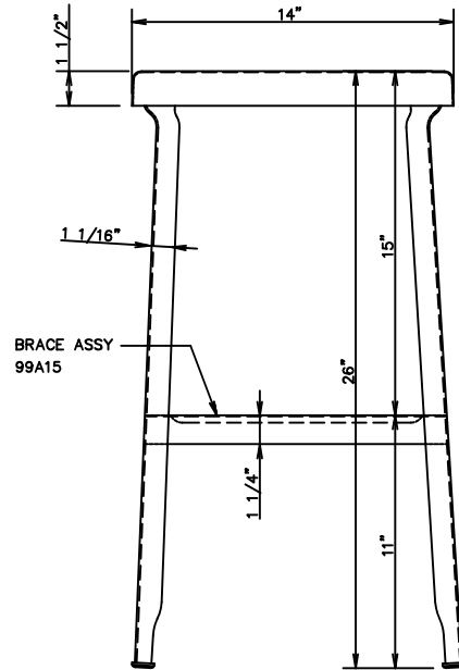
26" STOOL ASSY. NUMBER: 95A26
