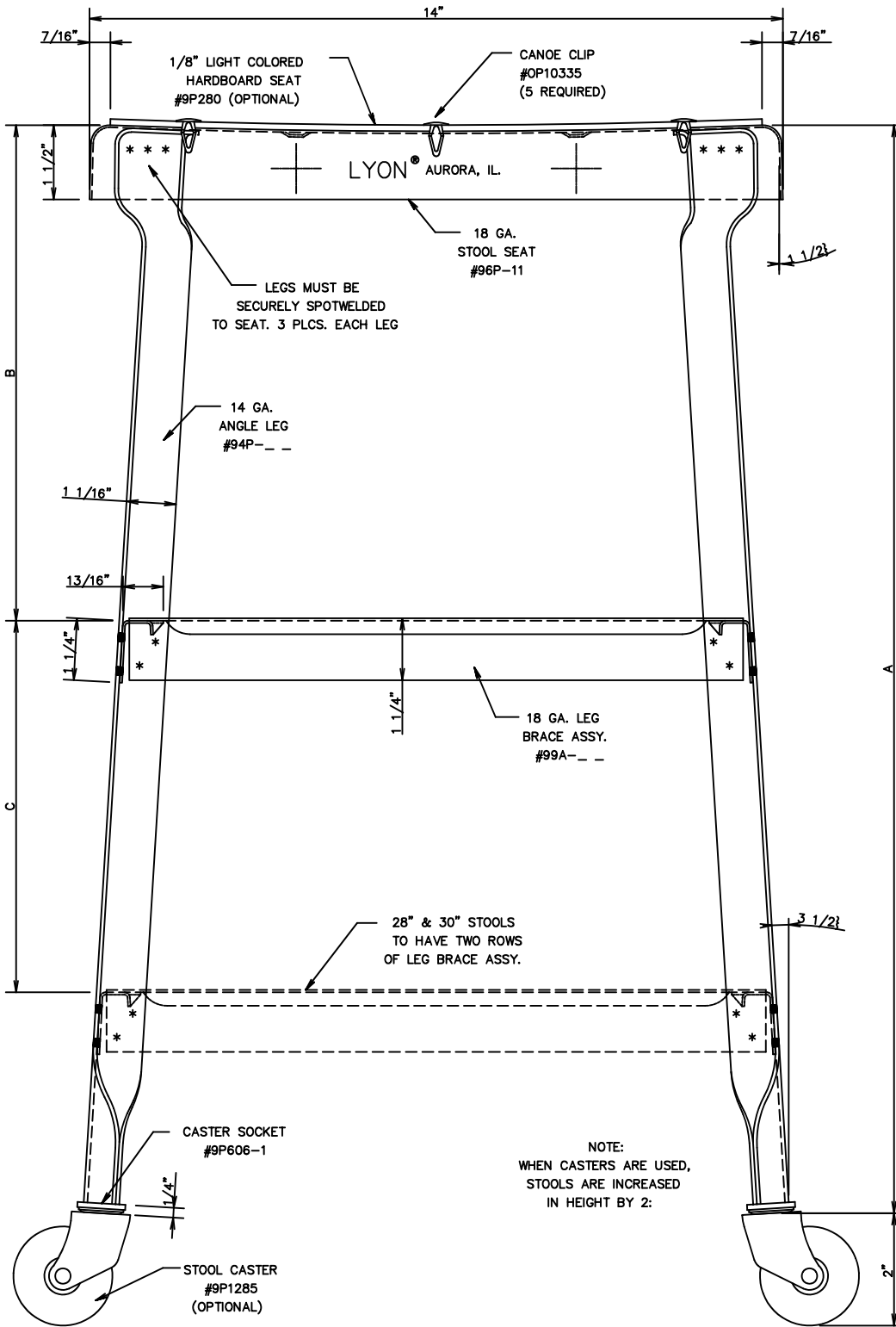
VERTICAL SECTION THRU STOOL
