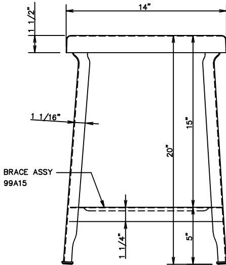
20" STOOL ASSY. NUMBER: 95A20
