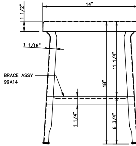
18" STOOL ASSY. NUMBER: 95A18
