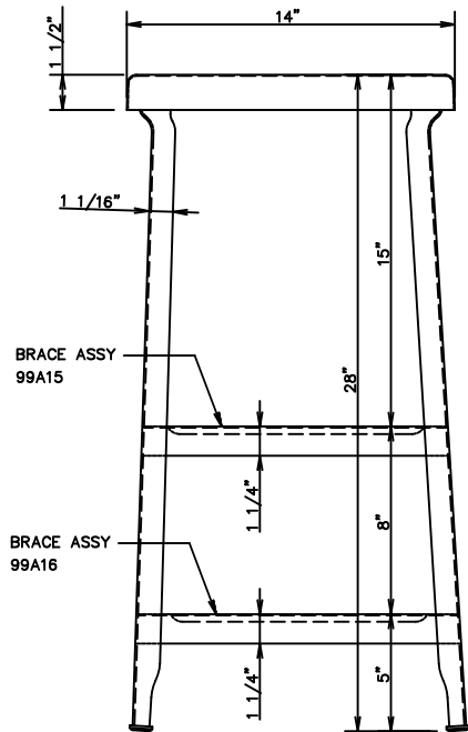
28" STOOL ASSY. NUMBER: 95A28
