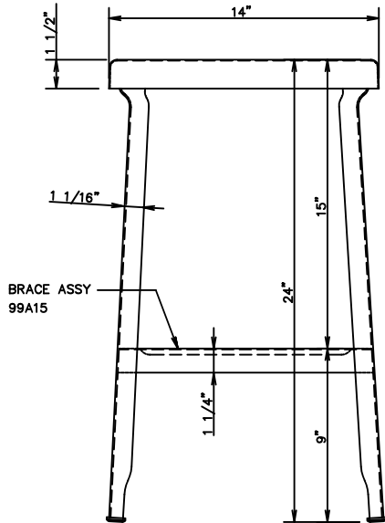
24" STOOL ASSY. NUMBER: 95A24
