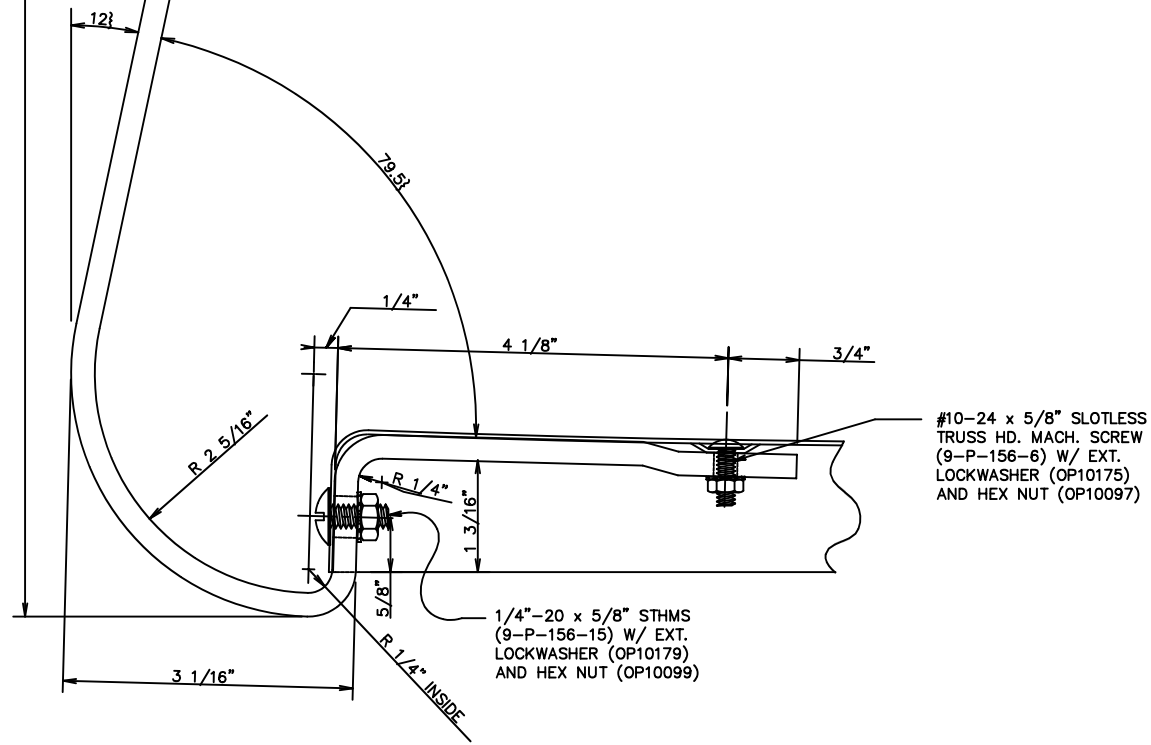
VERTICAL SECTION THRU STOOL BACK
