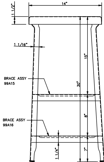
30" STOOL ASSY. NUMBER: 95A30
