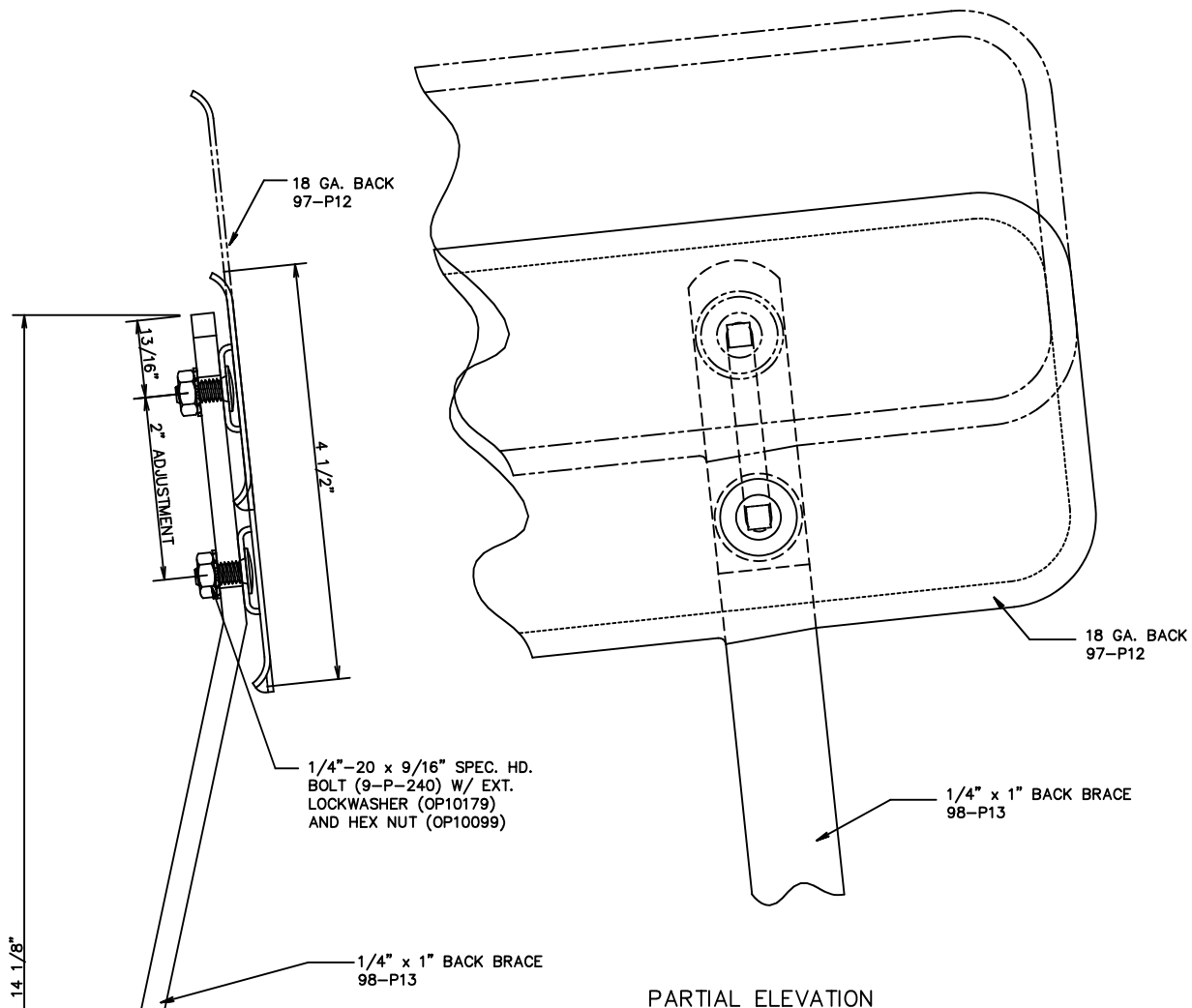
PARTIAL ELEVATION
