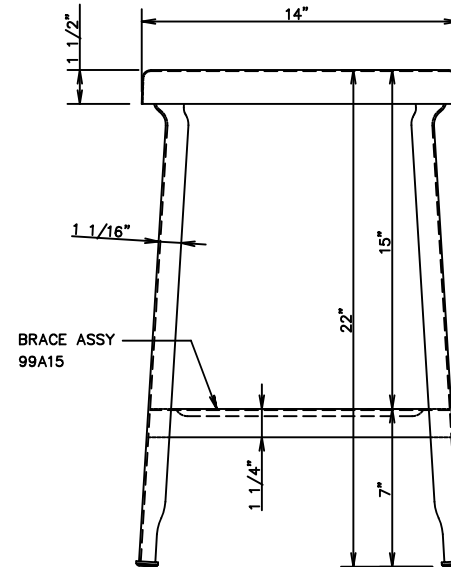
22" STOOL ASSY. NUMBER: 95A22
