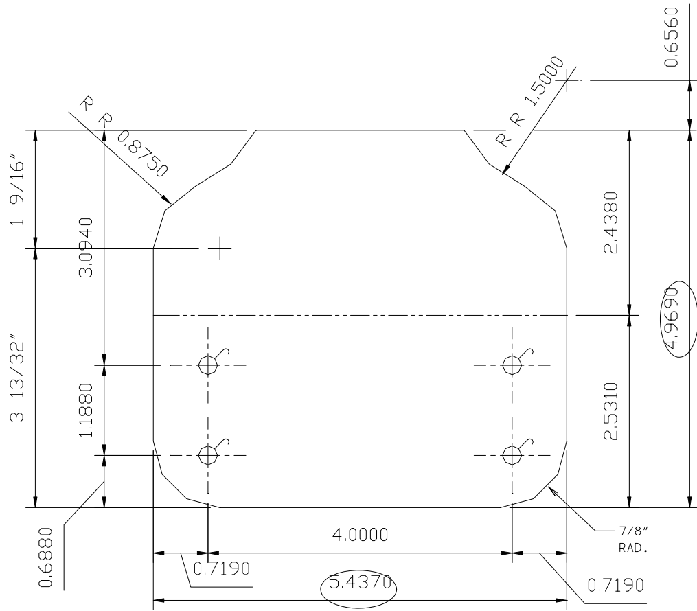
#14 GA. (H.R.P.) BENCH LEG FOOT PART NUMBER 3154-P-
