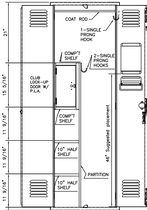
FRONT ELEVATION w/ DOORS OPEN
