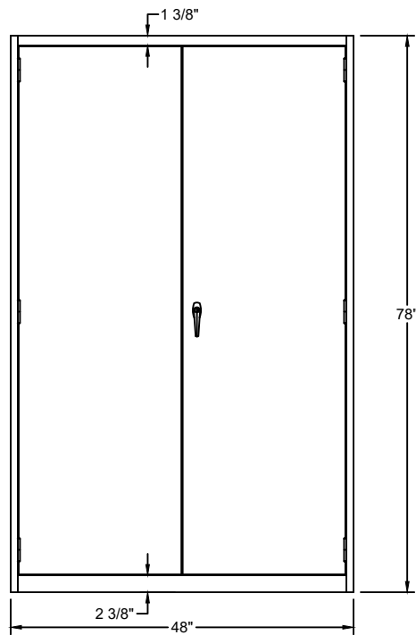
FRONT ELEVATION
