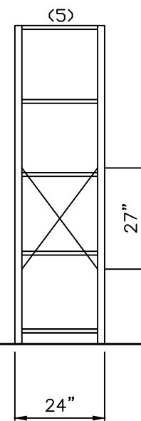
SIDE VIEW 24" x 84"
