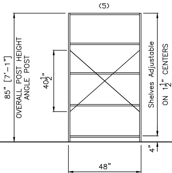
FRONT VIEW 48" x 84" 5 SHELVES
