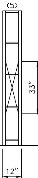
SIDE VIEW 12" x 84"
