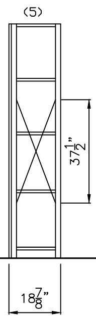
SIDE VIEW 18" x 84"
