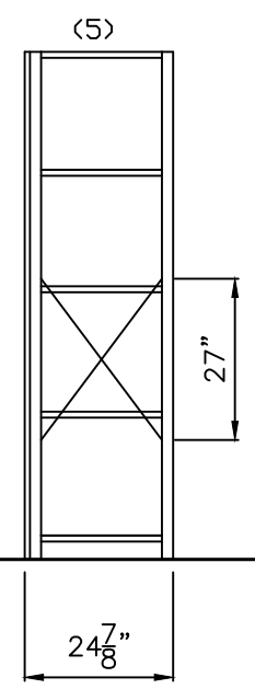
SIDE VIEW 24" x 84"
