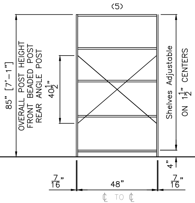
FRONT VIEW 48" x 84" 5 SHELVES
