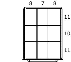
DRAWER LAYOUT "0C" 9 COMPARTMENTS
