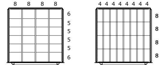
DRAWER LAYOUT "0E" 24 COMPARTMENTS
