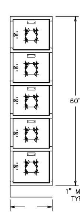
FRONT ELEVATION
