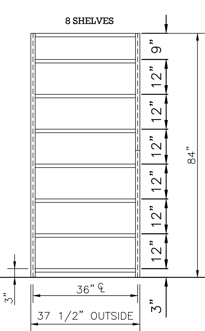
FRONT VIEW Shelves are adjustable on 1-1/2" Centers 36" X 84"
