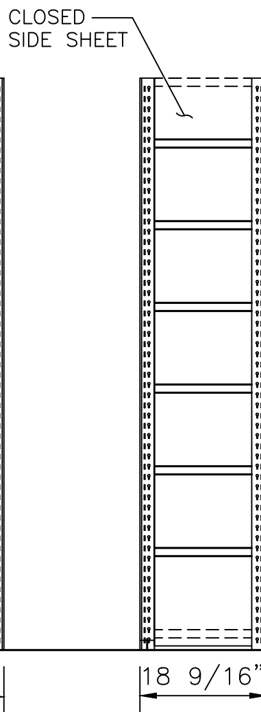
SIDE VIEW 18" X 84"
