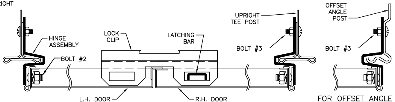
DETAIL "B"
