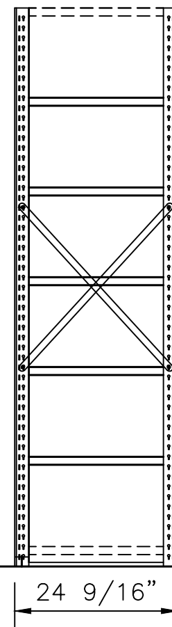
SIDE VIEW 24" X 84"
