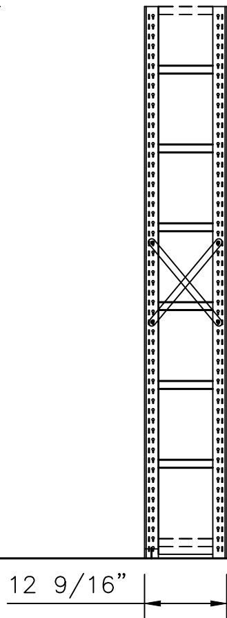
SIDE VIEW 12" X 84"
