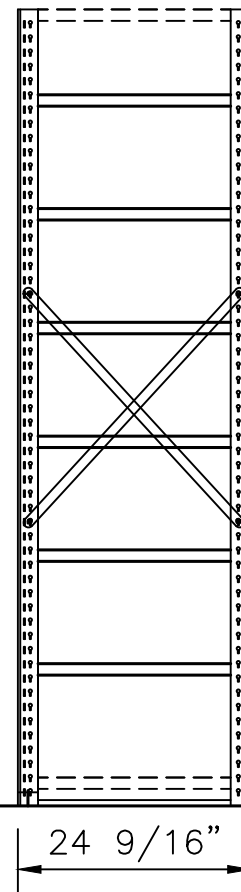
SIDE VIEW 24" X 84"
