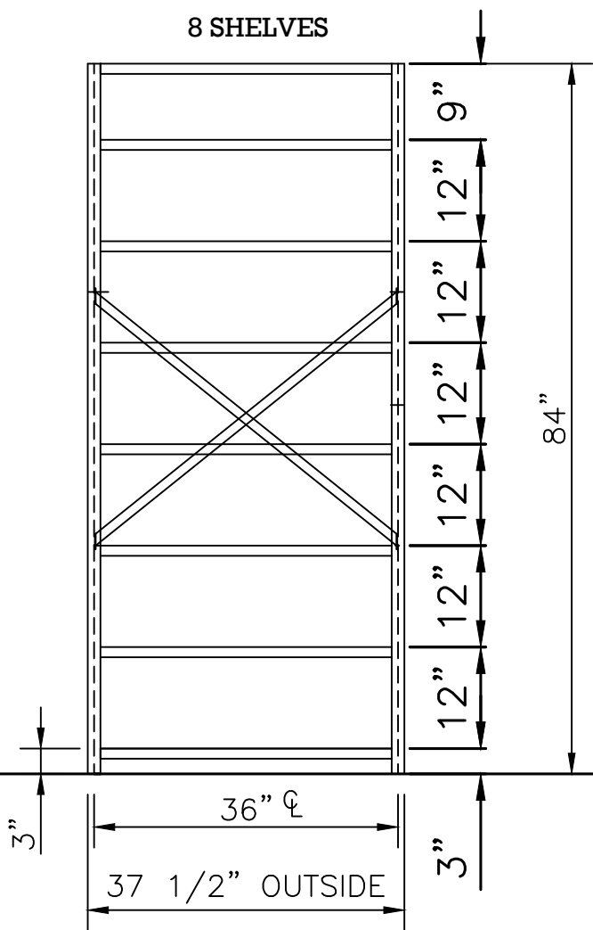
FRONT VIEW Shelves are adjustable on 1-1/2" Centers 36" X 84"
