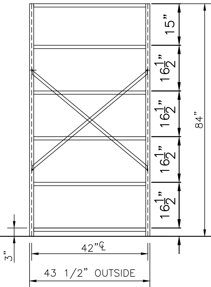
FRONT VIEW Shelves are adjustable on 1-1/2" Centers 42" X 84"
