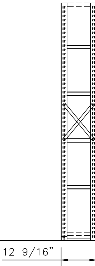
SIDE VIEW 12" X 84"
