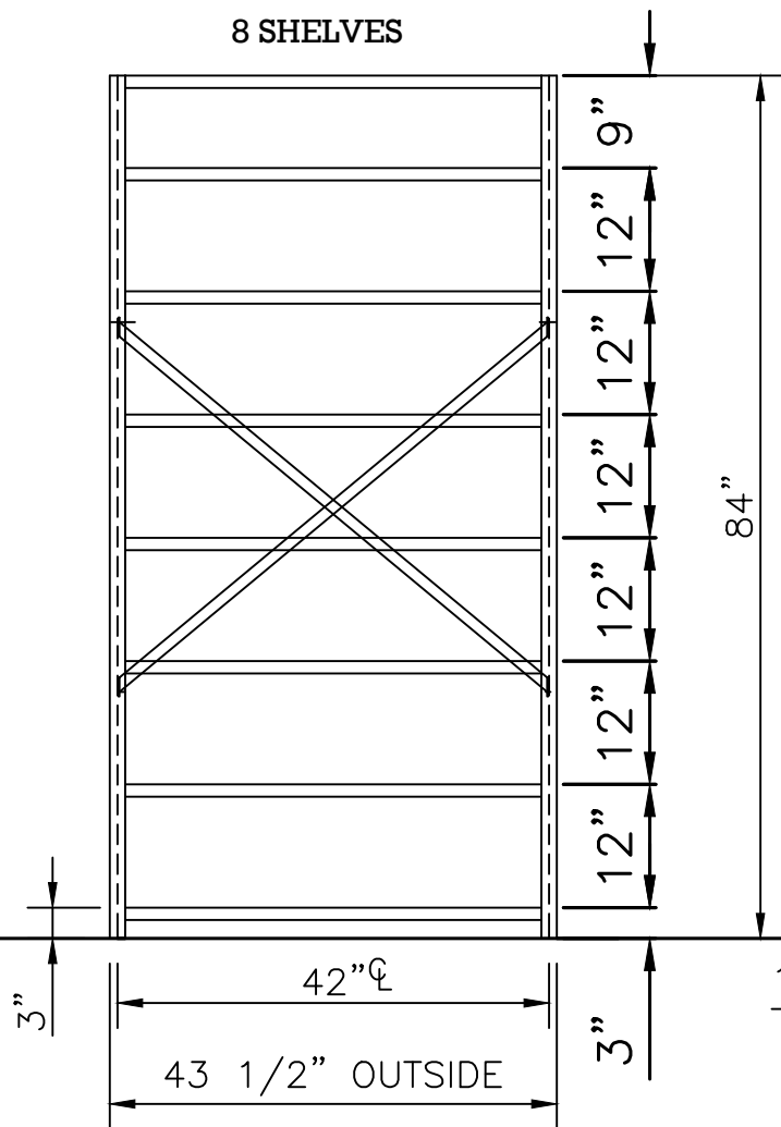
FRONT VIEW Shelves are adjustable on 1-1/2" Centers 42" X 84"
