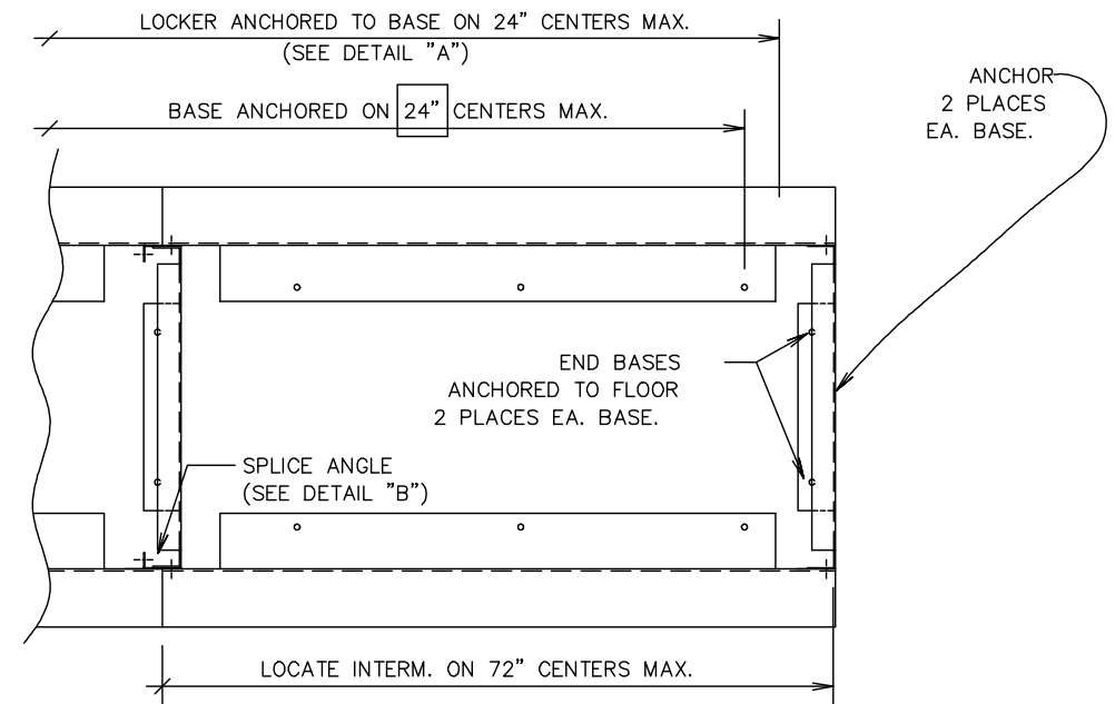
PARTIAL PLAN VIEW OF "Z" BASE
