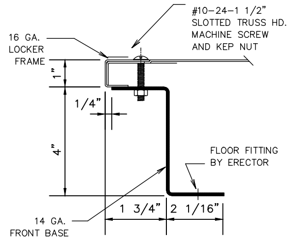
DETAIL "A" -FRONT BASE-
