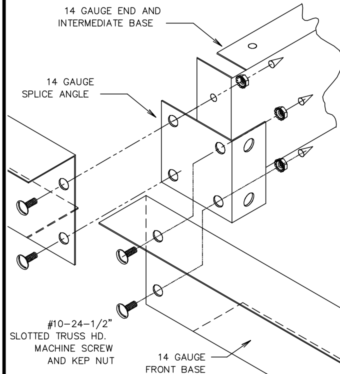
DETAIL "B"
