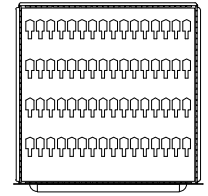
DRAWER LAYOUT "PSF2" 64 PISTOLS
