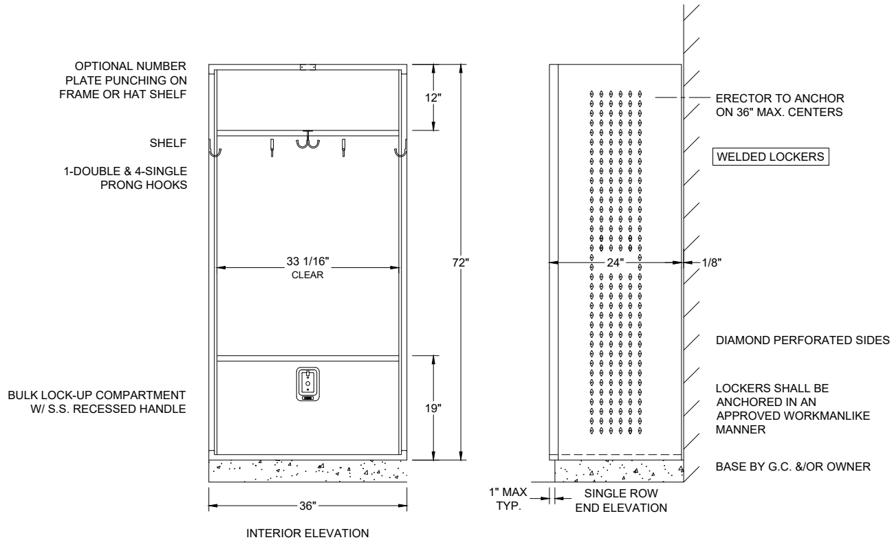
ALL WELDED COLLEGIATE LOCKER FRAME 36" X 24" X 72" S.R.S.T.
