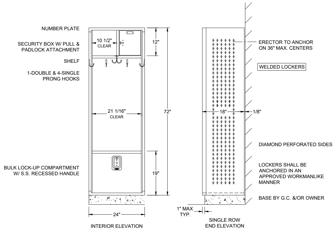
ALL WELDED DELUXE COLLEGIATE LOCKER FRAME 24" X 18" X 72" S.R.S.T.
