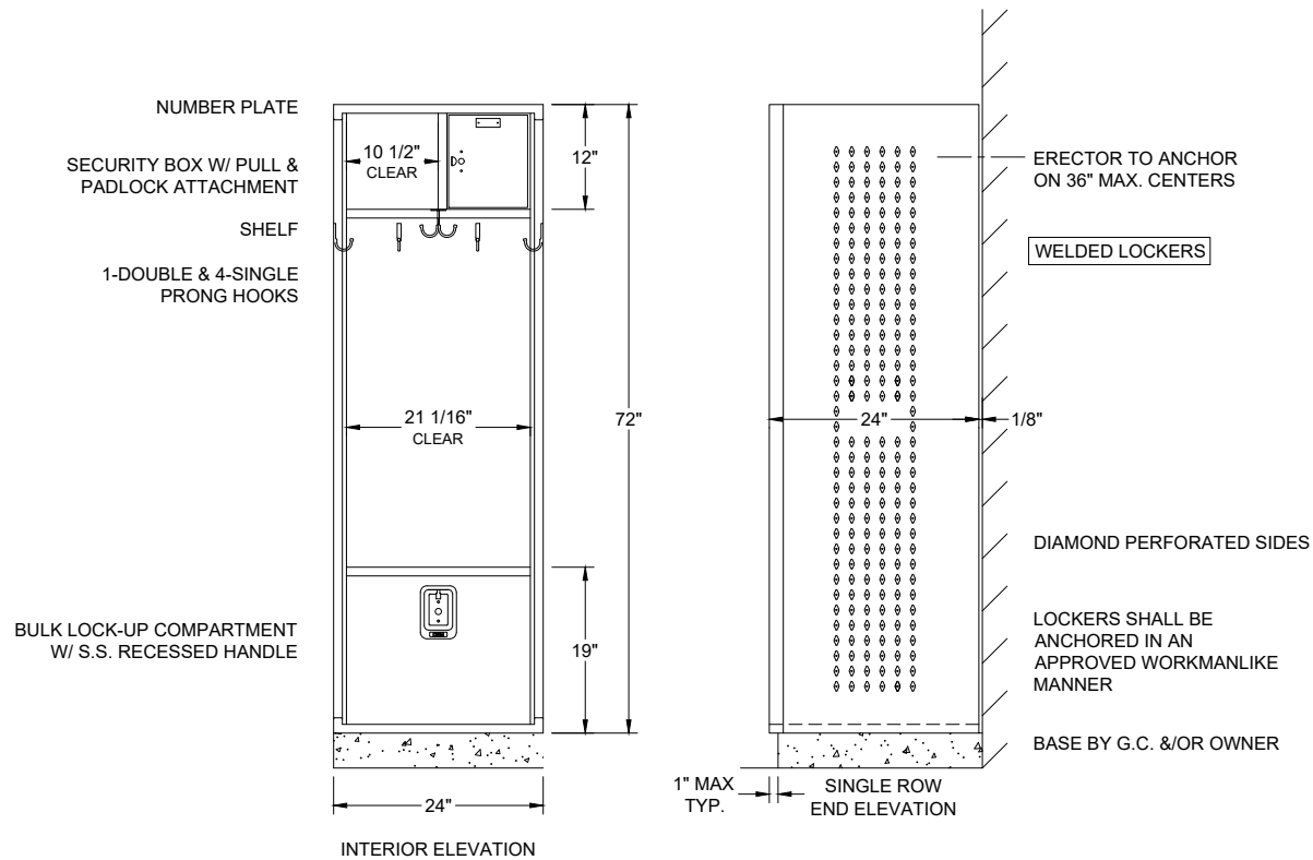
ALL WELDED DELUXE COLLEGIATE LOCKER FRAMES 24" X 24" X 72" S.R.S.T.
