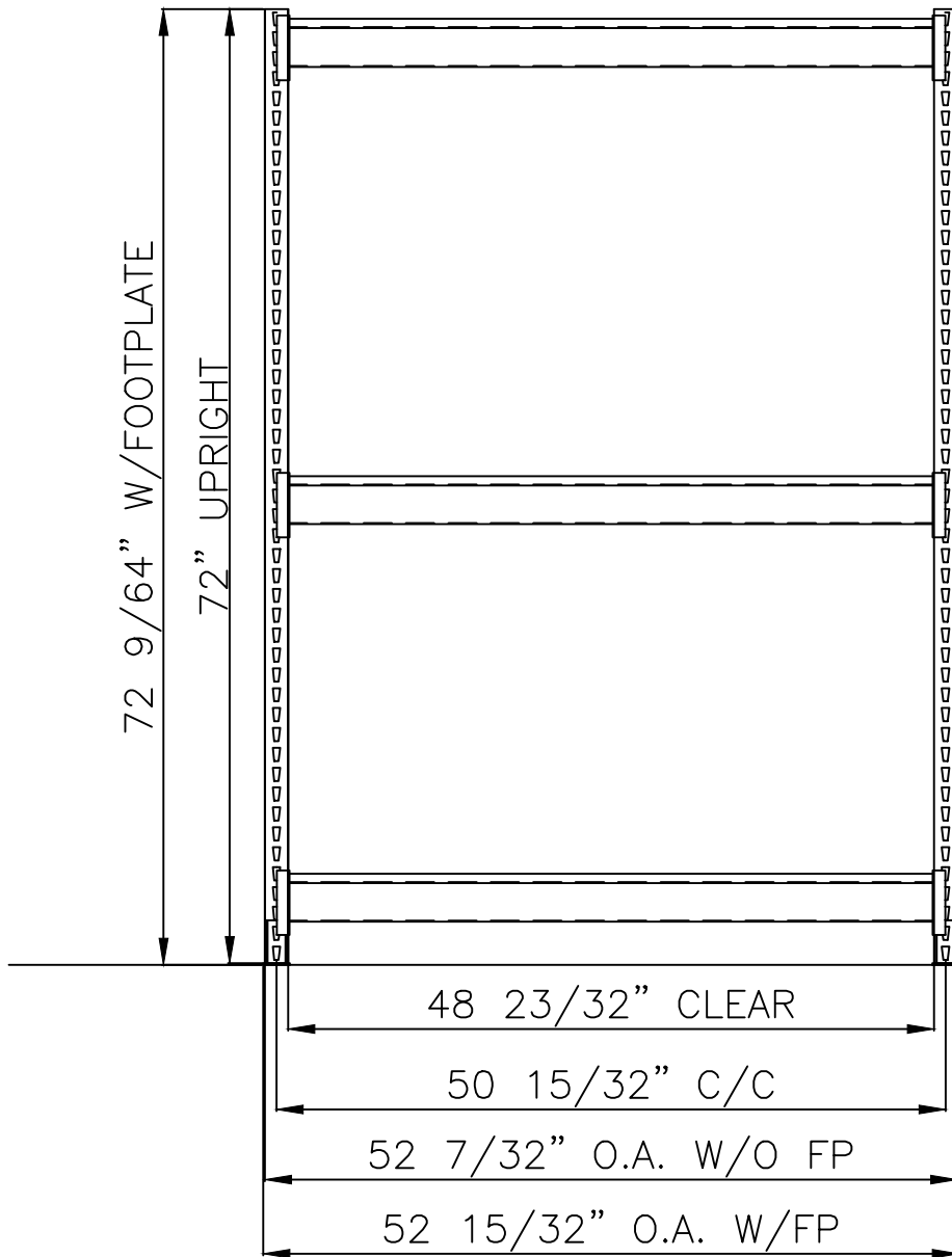
FRONT VIEW
