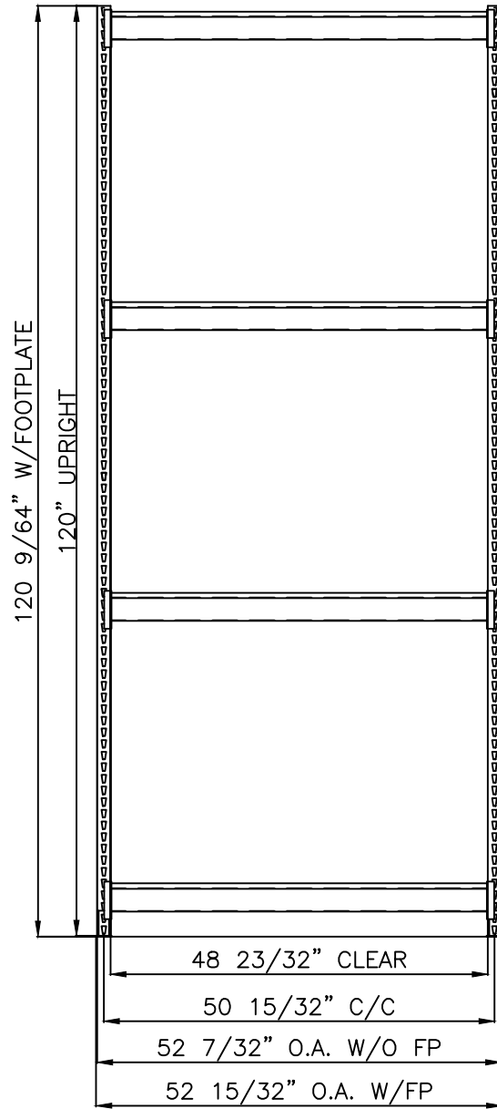
FRONT VIEW
