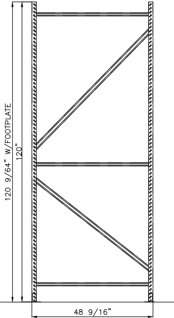
SIDE VIEW
