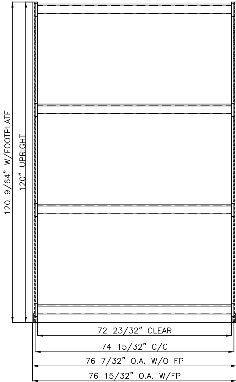
FRONT VIEW
