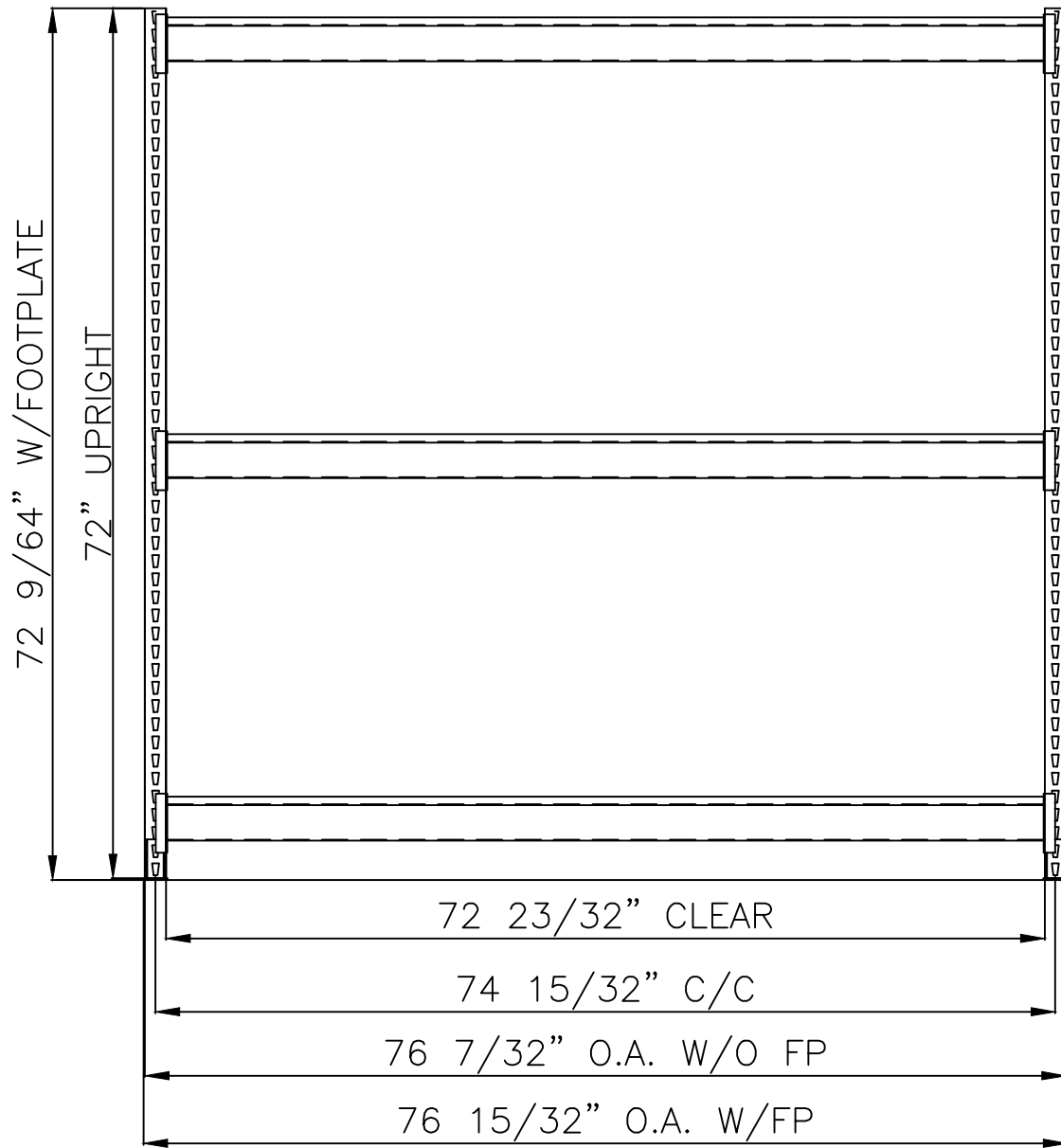
FRONT VIEW
