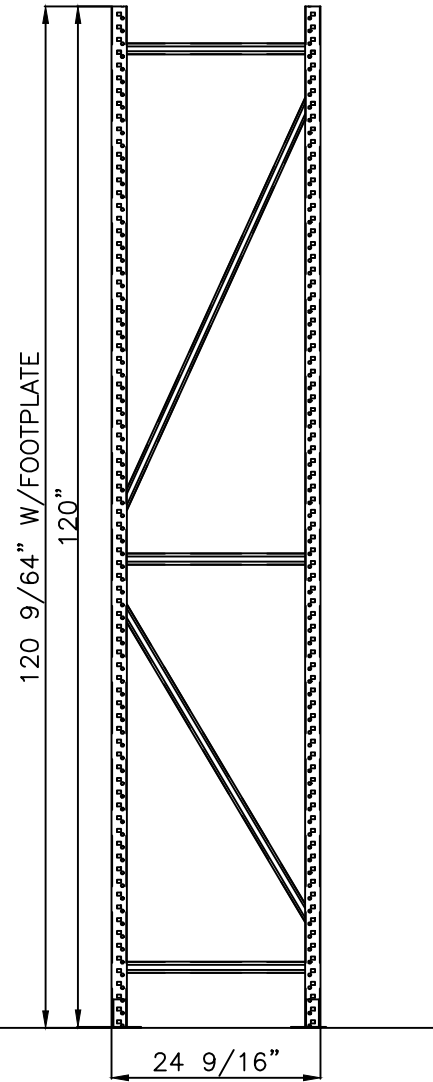
SIDE VIEW
