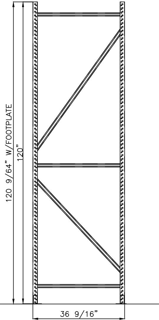
SIDE VIEW
