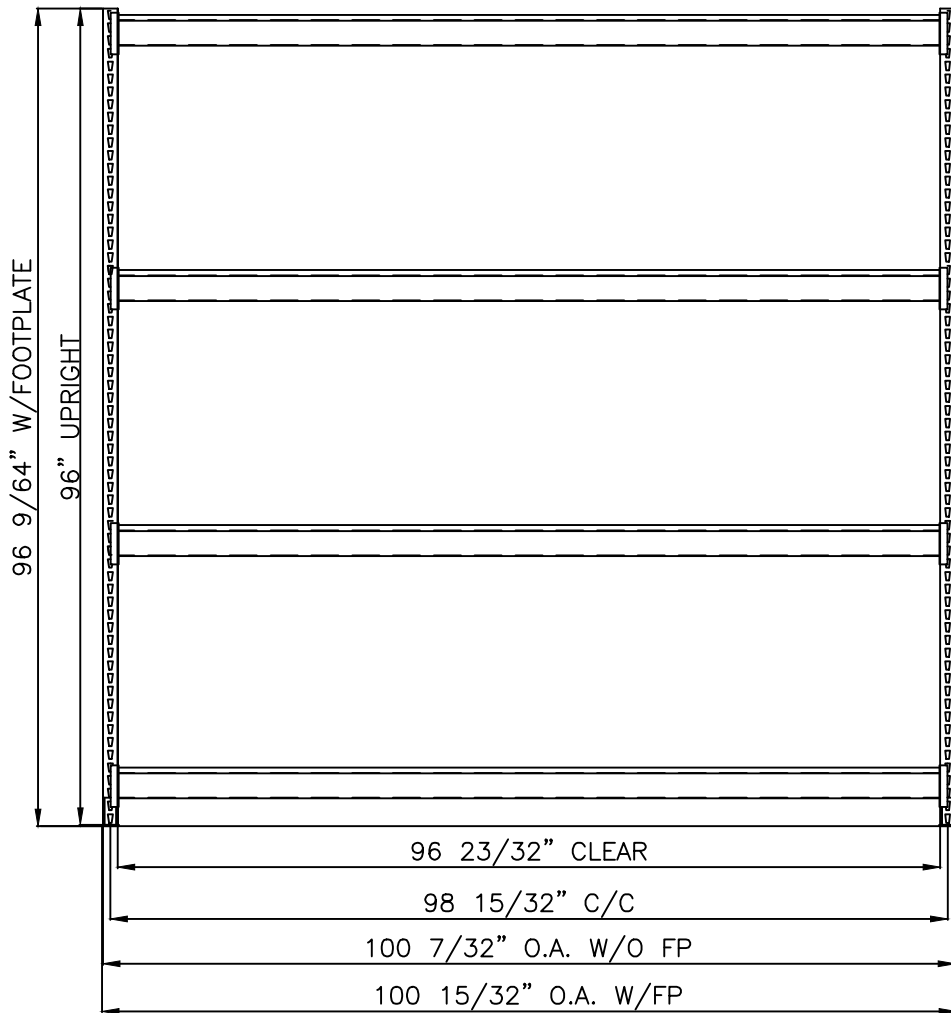
FRONT VIEW
