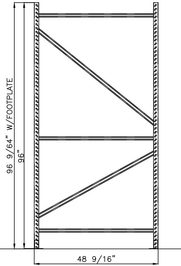
SIDE VIEW
