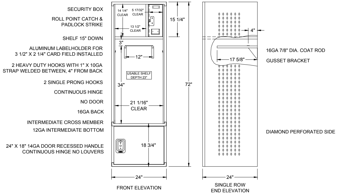
WELDED COMMAND GEAR LOCKER FRAME 24" X 24" X 72" S.R.S.T.
