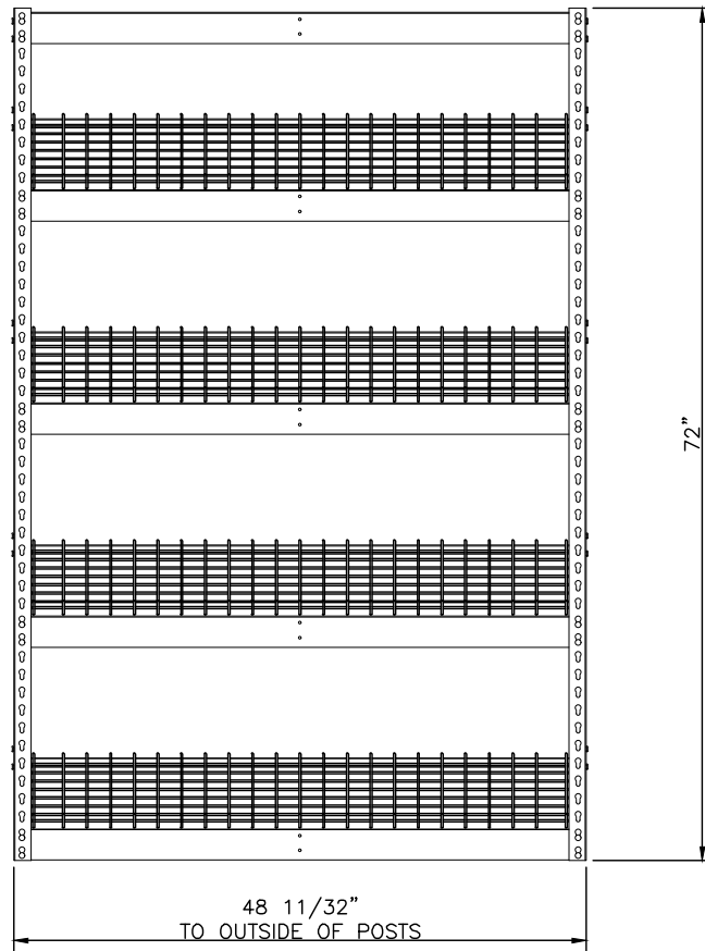
48" x 36" x 72" 4-LEVEL BATTERY RACK DDBR483672
