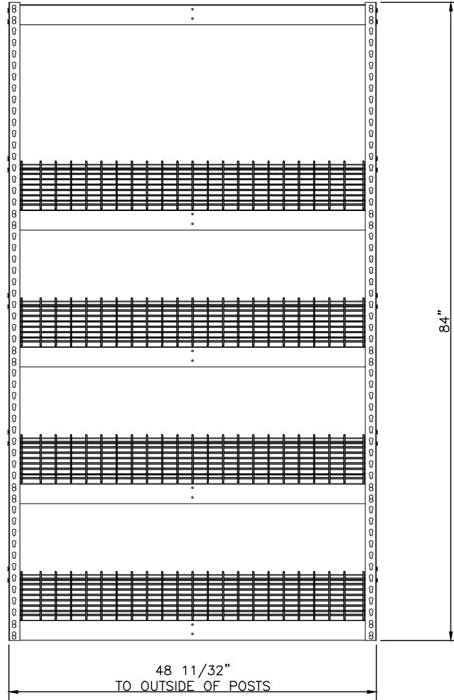
48" x 36" x 84" 4-LEVEL BATTERY RACK DDBR483684
