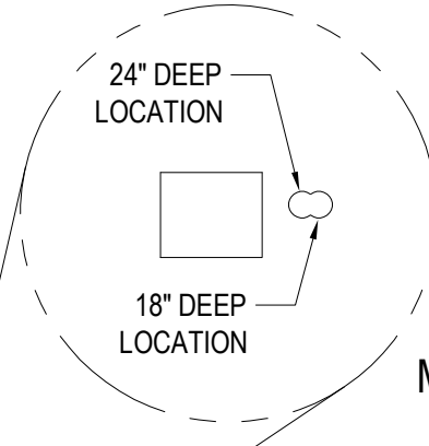
DETAIL SHOWING FRONT BRACKET PUNCHING (RIGHT HAND SHOWN)
