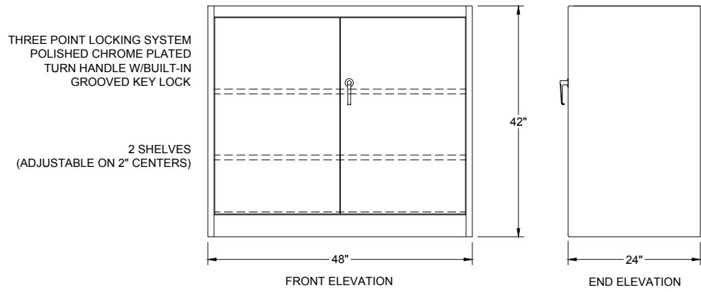
LYON 1000 SERIES STORAGE CABINET CAT# 1035SU SET-UP UNIT 48"W x 24"D x 42"H COLOR: _____
