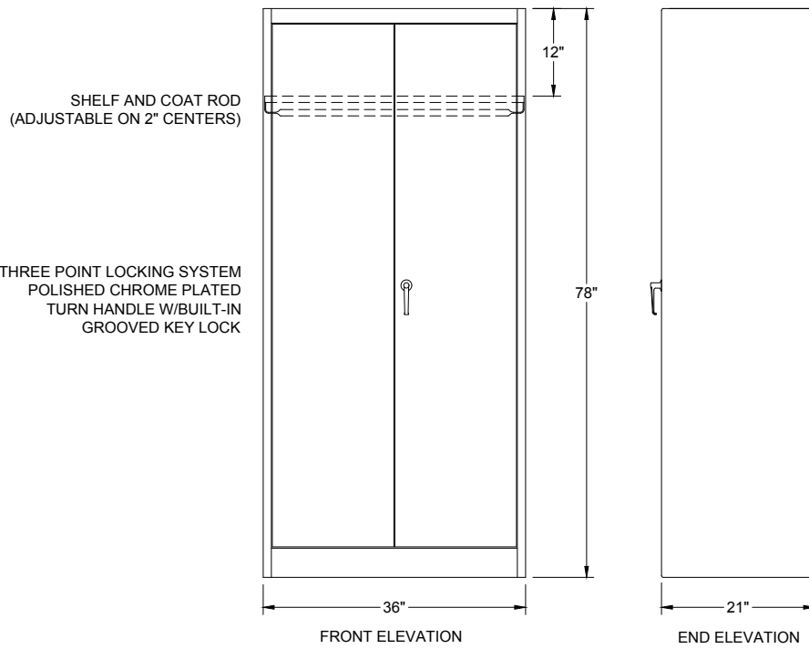
LYON 1000 SERIES WARDROBE CABINET CAT# 1005 SET-UP UNIT - 36"W x 21"D x 78"H COLOR: _____
