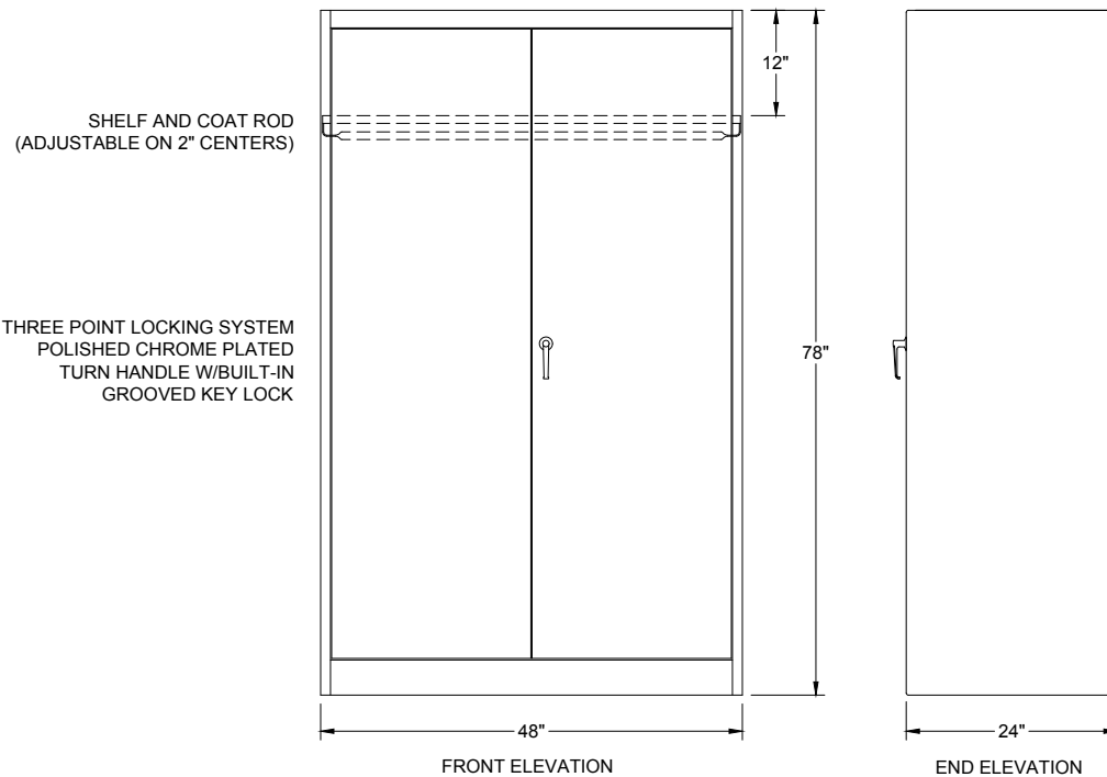
LYON 1000 SERIES WARDROBE CABINET CAT# 1032SU SET-UP UNIT - 48"W x 24"D x 78"H COLOR: _____
