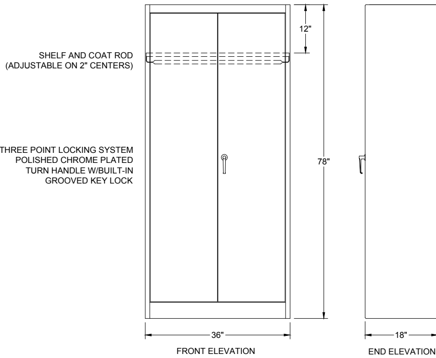
LYON 1000 SERIES WARDROBE CABINET CAT# 1085 SET-UP UNIT - 36"W x 18"D x 78"H COLOR: _____
