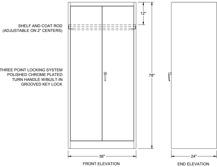
LYON 1000 SERIES WARDROBE CABINET CAT# 1095 SET-UP UNIT - 36"W x 24"D x 78"H COLOR: _____
