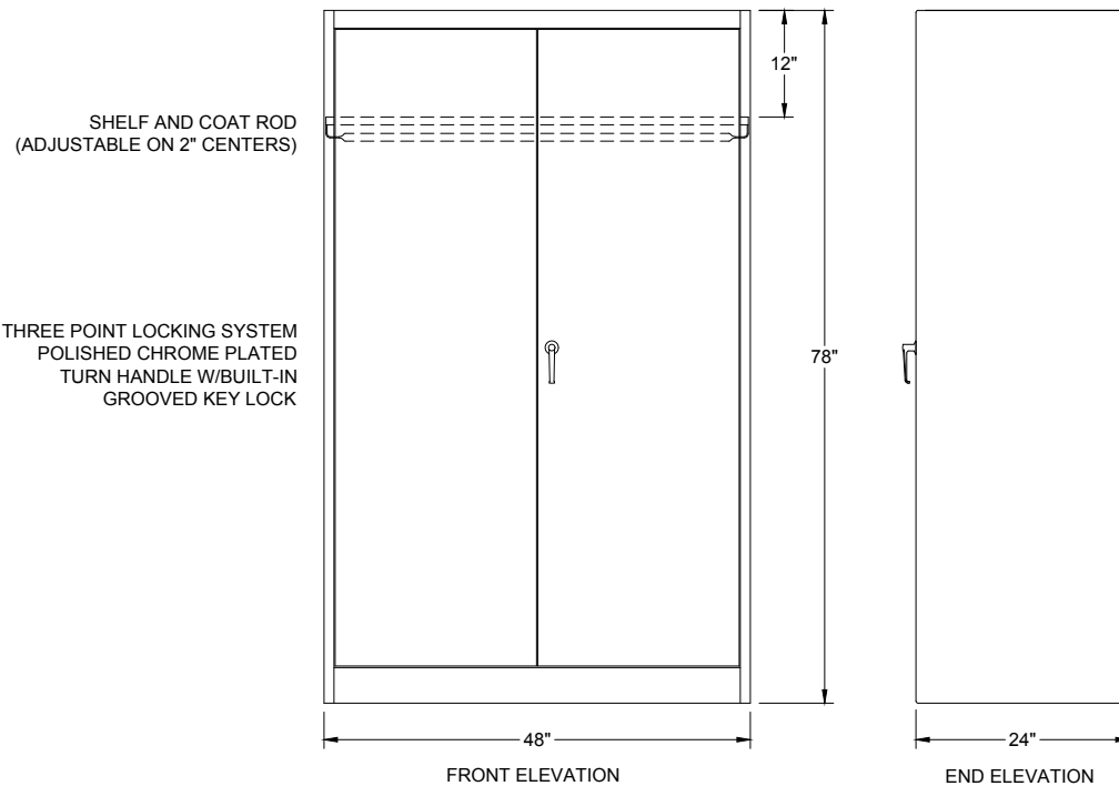
LYON 1000 SERIES WARDROBE CABINET CAT# 1032 KNOCK DOWN UNIT - 48"W x 24"D x 78"H COLOR: _____
