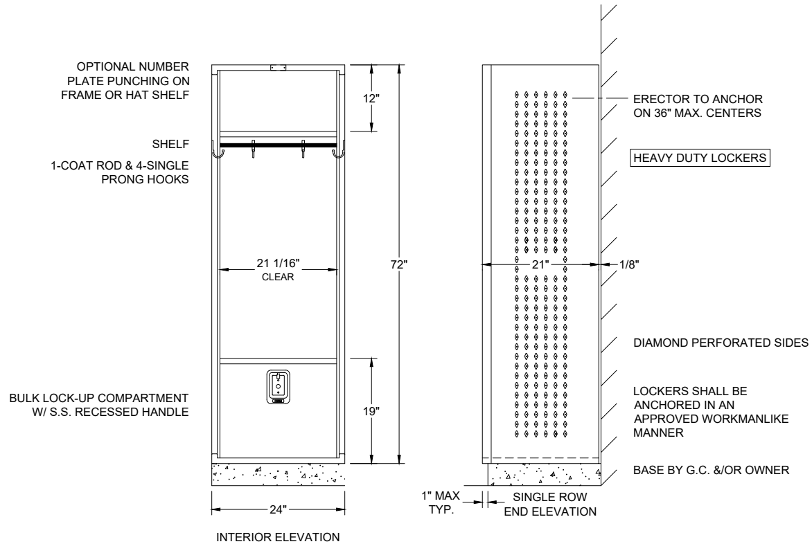
HEAVY DUTY COLLEGIATE LOCKER FRAME 24" X 21" X 72" S.R.S.T.
