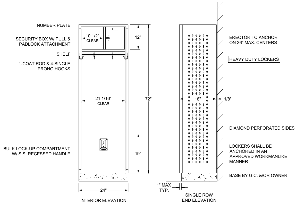
HEAVY DUTY DELUXE COLLEGIATE LOCKER FRAME 24" X 18" X 72" S.R.S.T.
