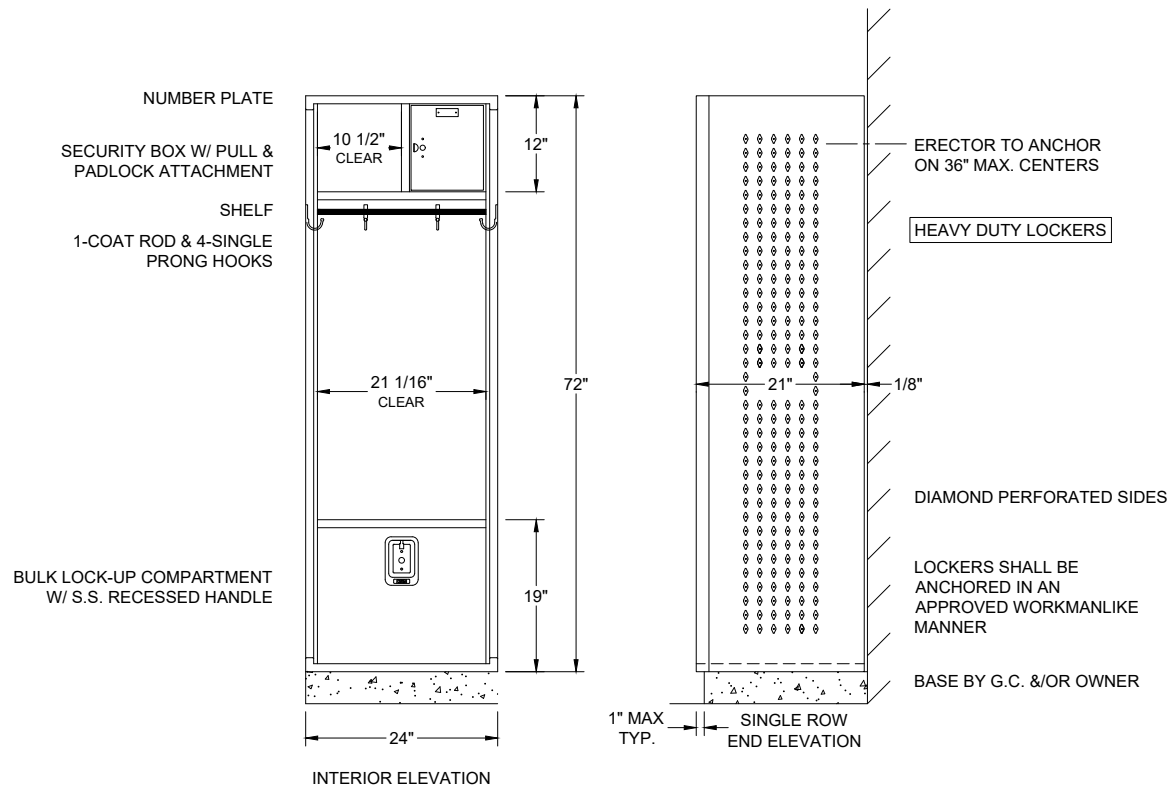
HEAVY DUTY DELUXE COLLEGIATE LOCKER FRAME 24" X 21" X 72" S.R.S.T.
