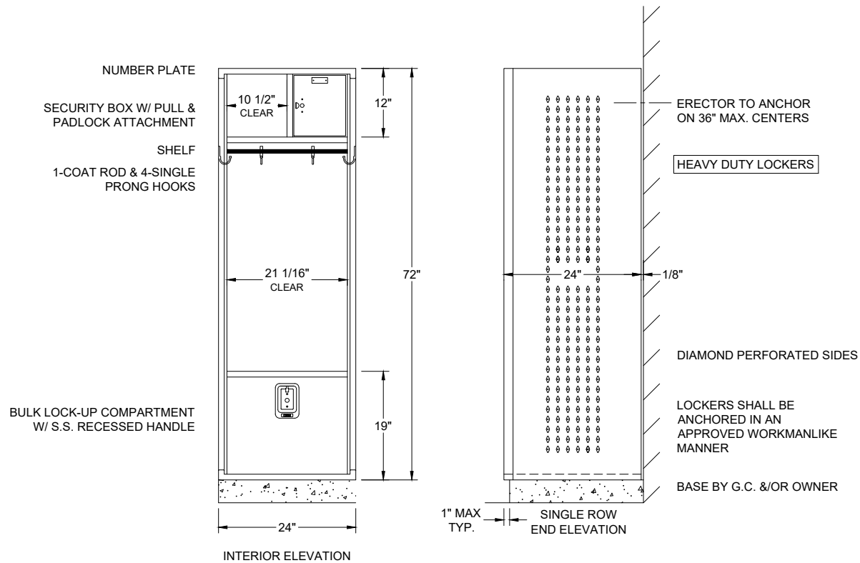
HEAVY DUTY DELUXE COLLEGIATE LOCKER FRAME 24" X 24" X 72" S.R.S.T.
