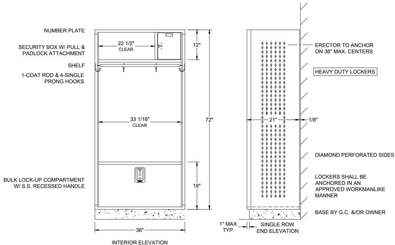
HEAVY DUTY DELUXE COLLEGIATE LOCKER FRAMES 36" X 21" X 72" S.R.S.T.
