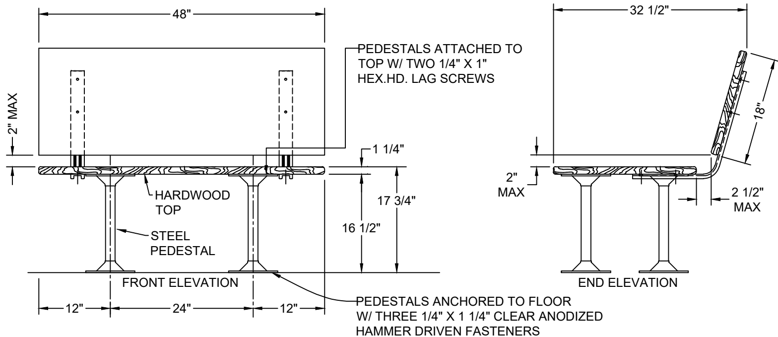
1 ADA BENCH 48" LONG X 24" DEEP W/ BACK REST
