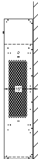
SINGLE ROW END ELEVATION
