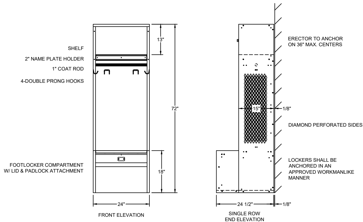
XXV452C VICTORY LOCKER FRAMES 24" X 24 1/2" X 72" S.R.S.T.
