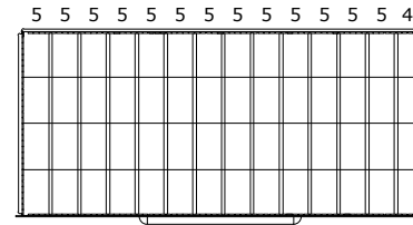
DRAWER LAYOUT "AU" 56 COMPARTMENTS
