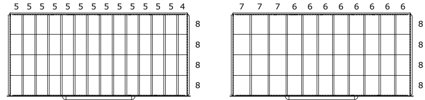
DRAWER LAYOUT "AU" 56 COMPARTMENTS
