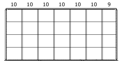
DRAWER LAYOUT "AR"
