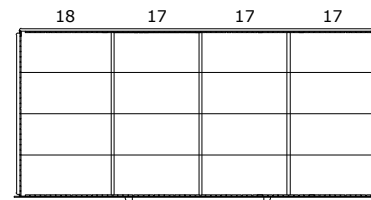
DRAWER LAYOUT "OP" 16 COMPARTMENTS
